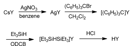
Scheme 1. Synthesis of the carborane acid HY (Y = CHB 11 F 11 − ).
